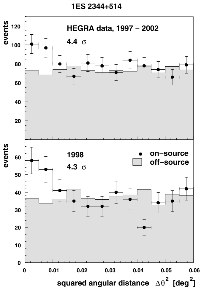
Fig. 2. Distributions of reconstructed squared angular distances to the object direction (see text) of the IES 2344+514 data. The distribution of the on-source events is represented by the data points. The scaled background (off) is shown as a shaded histogram. The upper figure represents the total data set taken between 1997 and 2002 whereas the lower figure shows the 1998 data alone. As can be seen from this figure the excess accumulates essentially in the year 1998.
