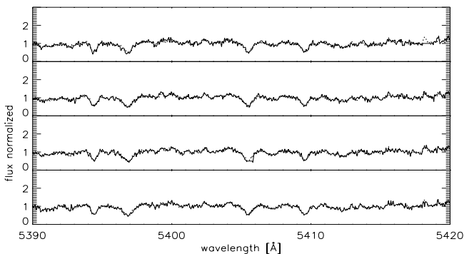
Fig. 4. Timeseries of a spectral range with several metal absorption lines. Clearly these photospheric lines are not affected by the blue shift seen in the chromospheric emission lines. Two cosmoics were removed manually by a horizontal line. The four pronounced absorption lines are due to Mn I (5394 Å), Fe I (5397 and 5405 Å) and Cr I (5409 Å). Again the dotted line denotes the time averaged spectrum.
