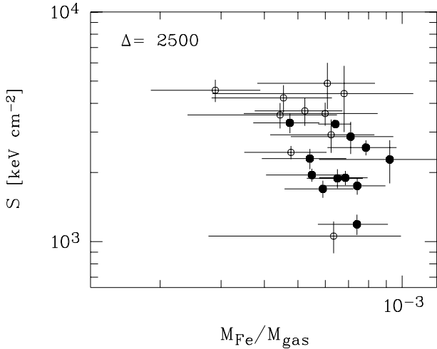
Fig. 13. Entropy versus iron abundance expressed in the form M_{\text{Fe}}/M_{\text{gas}} for CC (filled circles) and NCC (open circles) clusters. Both quantities are computed at overdensity 2500.
