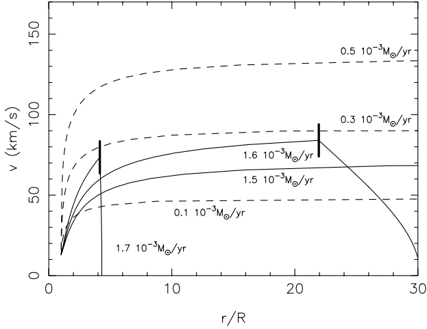
Fig. 4. Some velocity laws resulting from integration of the momentum equation for stellar parameters appropriate for \eta Car, allowing for different values of the velocity gradient at the sonic point. The full lines are solutions for the polar region while the dashed lines are valid for the equatorial regions. The mass-loss rates corresponding to the velocity laws are indicated. For a more detailed explanation we refer to Paper I and to the text.
