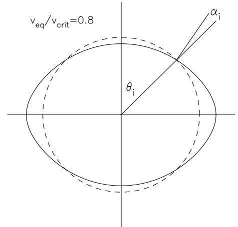
Fig. 2. A rotationally distorted star according to the Roche model for v_{\text{eq}}/v_{\text{crit}} = 0.8 (full line). At a certain co-latitude \theta_i the surface normal to the distorted star encloses an angle \alpha_i with the radial vector, which is perpendicular to a spherical star with radius r(\theta_i) (dashed line). The surface-integrated maximum mass loss calculated from Exp. (5) takes into account the maximum mass flux along the normal to the true stellar surface.
