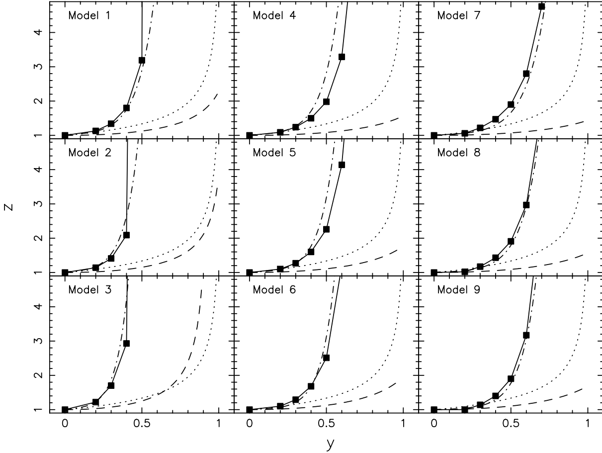
Fig. 3. z \equiv \dot{M}_{\max}^{\text{tot}}(v_{\text{eq}}/v_{\text{crit}})/\dot{M}_{\max}^{\text{tot}}(0) as a function of y \equiv v_{\text{eq}}/v_{\text{crit}} for rotating models including the Von Zeipel effect. The values are obtained from direct integration of the momentum equation at different co-latitudes and are indicated by filled boxes connected by a full line. The dotted line represents the empirical relation proposed by Langer (1998). The scaling law proposed by Maeder & Meynet (2000) for winds in rotating stars without instabilities is superimposed as a dashed line. The dashed-dotted line represents the multiple regression prediction formula given in Exps. (8) and (9).
