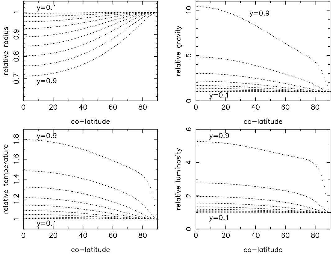
Fig. 1. The local radius ( upper left ), local gravity ( upper right ), local effective temperature ( lower left ) and local luminosity L(\theta) \equiv 4\pi R^2(\theta)T_{\text{eff}}^4(\theta) ( lower right ) relative to the equatorial value of these quantities, for different ratios of the equatorial velocity to the critical velocity and as a function of co-latitude ( \theta = 0 at the pole). The step in y = v_{\text{eq}}/v_{\text{crit}} for the different dotted curves is 0.1.
