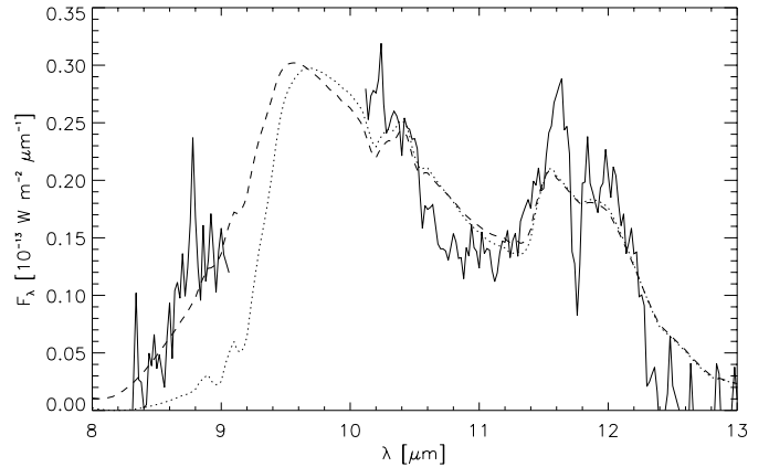
Fig. 11. Fit to the continuum-subtracted spectrum of IRAS 05358–0238. The dotted line represents a self-absorbed forsterite profile, while the dashed line further includes a contribution from small grains of amorphous silicate (see text).
