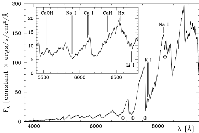
Fig. B.1. Optical spectrum of IRAS 05358–0238. Several atomic and molecular features are identified. The inset shows the absence of CaOH and CaH, which suggests this object to be a giant.
