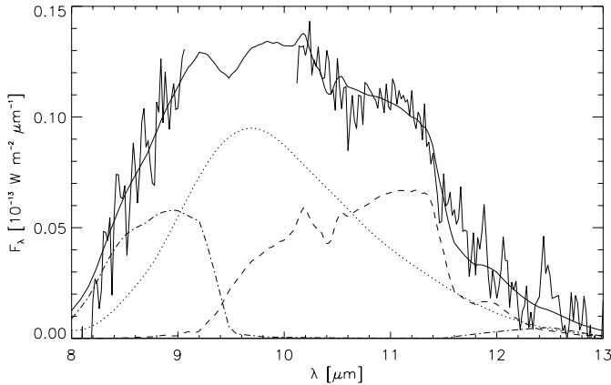
Fig. 10. Fit to the continuum-subtracted spectrum of TX Ori. The solid line is the best-fit model spectrum, the dotted line is the (small grain) amorphous silicate contribution and the dashed and dashed-dotted lines are the contributions of the crystalline species, respectively forsterite and silica.
