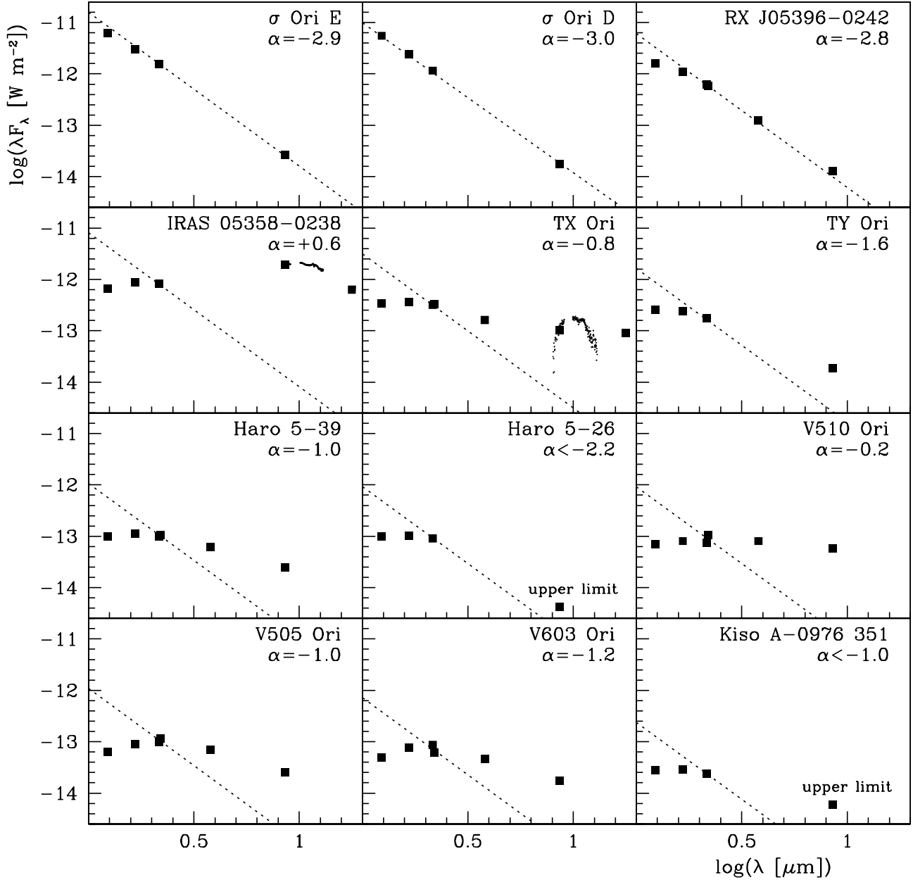
Fig. 4. Infrared spectral energy distributions for all targets except \sigma Orionis and \sigma Ori IRS1, ordered in luminosity (from left to right and from top to bottom). The spectral index is defined as \alpha = (F_{N1} - F_K)/(\lambda_{N1} - \lambda_K) , and the dotted line through the K -band point is for \alpha = -3 . Objects with \alpha \geq -2 are believed to possess dusty circumstellar material.
