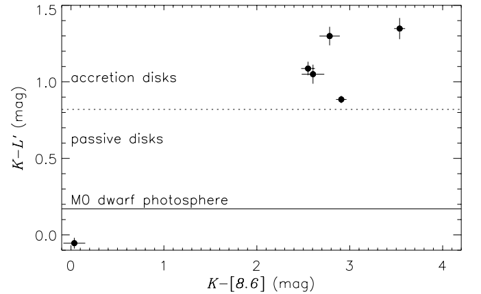
Fig. 8. KL'NI colour–colour diagram. The solid line corresponds to the K - L' colour of a main-sequence star with M0 spectral type. The dotted line separates passive from accretion disks, for a K7–M0 star, according to Wood et al. (2002).
