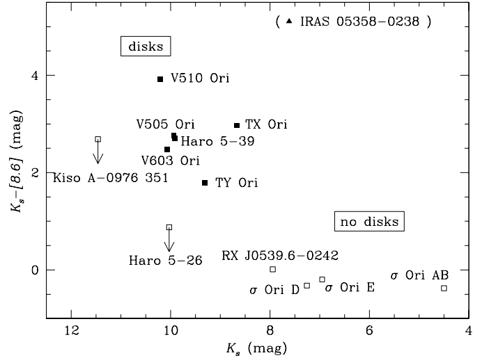
Fig. 7. The (K_s - [8.6]) vs. K_s colour–magnitude diagram for stars with (filled symbols) and without (open symbols) disks. There is a clear separation between brighter diskless objects and fainter objects with evidence of circumstellar material.
