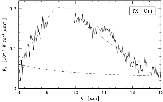
Fig. 5. N -band spectrum of TX Ori. Using the procedure described in the text, the 10\ \mu\text{m} feature is shown to closely resemble the so-called “Trapezium emissivity” (dotted line), i.e. it is readily identified as a silicate emission feature. There is, however, an extra feature at about 11.2\ \mu\text{m} . The dashed line is an estimate of the local continuum, as derived from the analysis of the SED (see Sect. 4.3).
