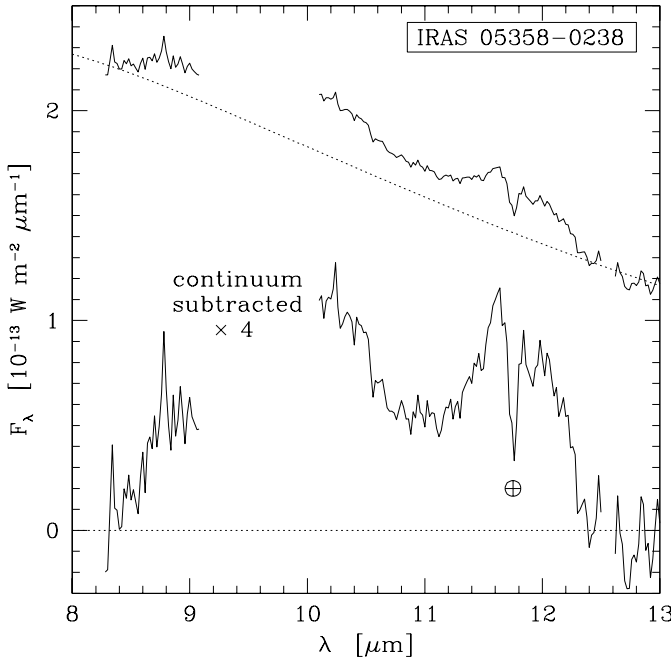
Fig. 6. N -band spectrum of IRAS 05358–0238. The dotted line on the top panel is an estimate of the local continuum, as derived from the analysis of the SED (see Sect. 4.4). The bottom panel shows the continuum-subtracted spectrum, which is highly unusual.
