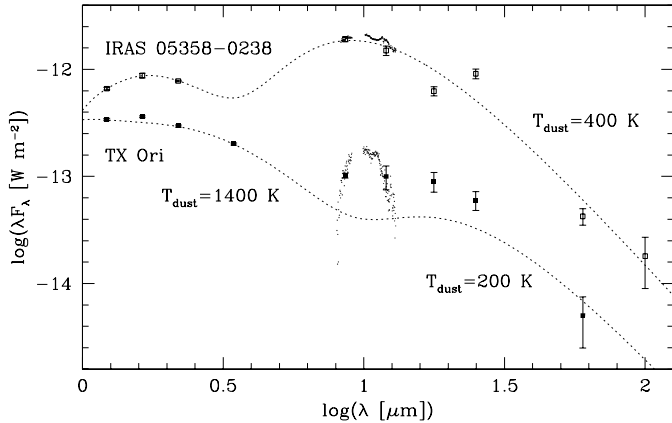
Fig. 9. Spectral energy distributions of IRAS 05358–0238 (open symbols) and TX Ori (solid symbols). The available IR fluxes allow us to estimate a typical temperature of the dust in the circumstellar environments of the two objects: respectively 400 K and 200 K for IRAS 05358–0238 and TX Ori. The K - and L -band fluxes of TX Ori require an additional warm dust component with a temperature \sim 1400 K. These simplified fits are used to estimate the continuum level in the region of the 10 \mu\text{m} feature.
