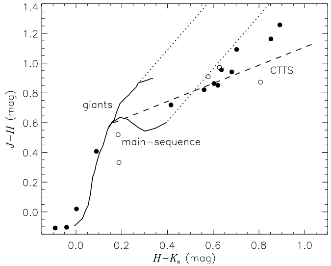
Fig. 3. JHK_s colour-colour diagram of targets of the TIMMI-2 observations, filled symbols are the objects effectively observed. The full lines are the loci of main-sequence and giant stars (Bessell & Brett 1988), the dotted lines are reddening bands (Bessell & Brett 1988; Rieke & Lebofsky 1985), the dashed line is the locus of classical T Tauri stars (Meyer et al. 1997), converted to the 2MASS photometric system (Carpenter 2001). Objects with colours to the right of the reddening band cannot be explained simply by photospheric emission from the star and suggest the presence of a circumstellar disk.
