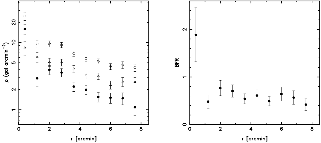
Fig. 7. Background-subtracted radial profile of ABCG 209 is shown in the left panel. Open circles represent the distribution of all galaxies in the cluster, filled circles are bright galaxies ( M_V^* \leq -19.5 ) and open triangles are faint galaxies ( M_V^* > -19.5 ). The number of bright galaxies in the first and in the second bin is \sim 32 and \sim 17 respectively, while the number of faint galaxies is \sim 15 and \sim 30 . The bright-to-faint ratio as a function of the clustercentric distance is shown in the right panel.
