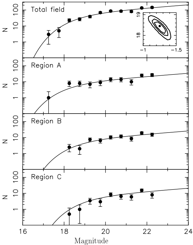
Fig. 6. Luminosity function in the V band. In the upper panel are shown the LF in the whole observed area ( 160 \text{ arcmin}^2 ) and the 1, 2 and 3\sigma c.l. of the best-fit parameters \alpha and M^* (small panel). The continuous line represents the fitted Schechter functions. In the other panels the LFs in the three cluster regions (see text) are shown. Continuous lines are the fit of the Schechter functions obtained by fixing the faint-end slope at the best fit value of the LF fitted on the whole observed area.
