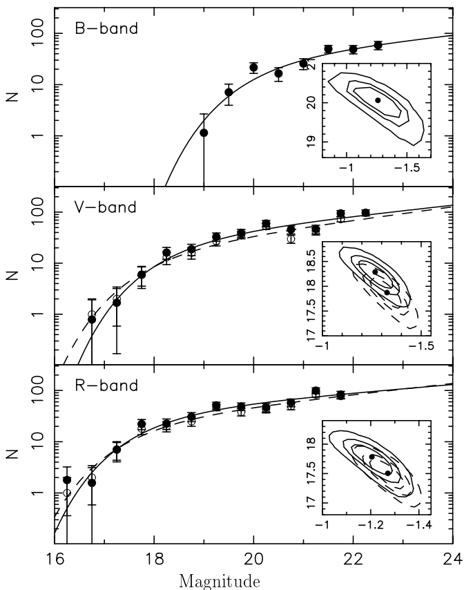
Fig. 3. Luminosity function in the B, V and R bands in the central field of 9.2' \times 8.6' . In V and R bands filled circles represent counts obtained from the photometric catalog with a statistical background subtraction, open circles are the counts of galaxies belonging to the red sequence of the CM relation (see Sect. 5.2). Solid and dashed lines are the Schechter fits to the filled and open circles respectively. In the small panels the 1, 2 and 3\sigma c.l. of the best-fit parameters \alpha and M^* are shown.
