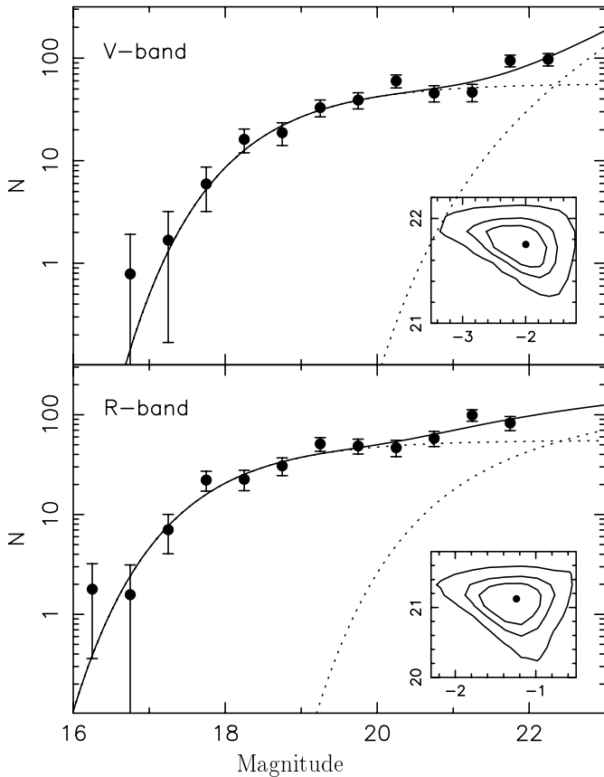
Fig. 4. Luminosity function in the V and R bands in the central field of 9.2' \times 8.6' . The dashed lines represent the Schechter functions for bright and faint galaxies separately (see text). The continuous line represents the sum of the two functions. In the small panels the 1, 2 and 3\sigma c.l. of the best-fit parameters \alpha and M^* are shown.
