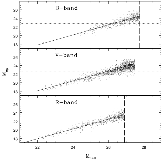
Fig. 2. Completeness magnitudes of the B -, V -, and R -band images are estimated by comparing magnitudes in the fixed aperture ( M_{\text{ap}} ) and in the detection cell ( M_{\text{cell}} ). The dotted lines represent the completeness limits, the dashed lines mark the limits in the detection cell, and solid lines are the linear relations between M_{\text{ap}} and M_{\text{cell}} .
