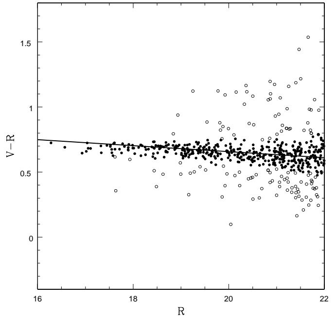
Fig. 5. V - R vs. R CM diagram for all the galaxies within the completeness limit in the central field of ABCG 209. Galaxies of the red sequence (see solid line) are plotted as filled circles. The solid line defines the CM sequence for spectroscopically confirmed cluster members.
