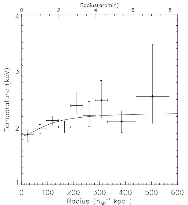
Fig. 5. The total XMM-EPIC radial temperature profile of A1983. The solid line is the best fit to the temperature profile with a function of the form given in Eq. (2). Errors are 1\sigma confidence level.
