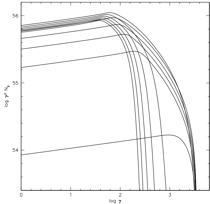
Fig. 5. Evolution of the electron energy distribution during the February 1996 flare of the blazar 3C 279. Step between the curves is \Delta r = 0.2 r_0 .
