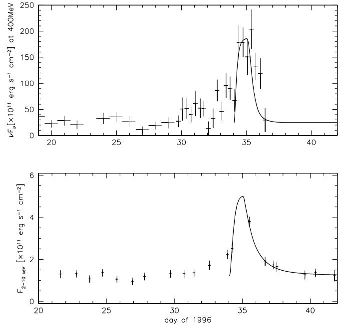
Fig. 3. \gamma -ray (upper panel – \nu F_\nu flux at 400 MeV) and X-ray (lower panel – integrated 2–10 keV flux) light-curves of the blazar 3C 279 during the February 1996 flare. Data points are from Wehrle et al. (1998). Thick, solid line shows the light-curves of our model.
