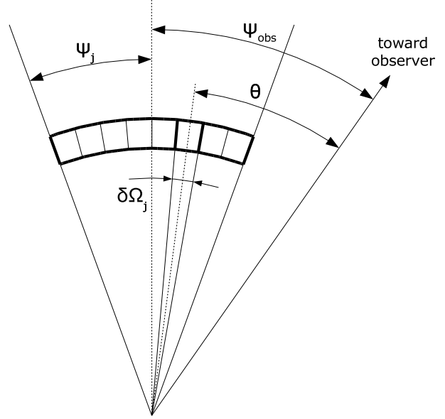
Fig. 1. A schematic picture illustrating the integration procedure. A thin shell of electrons enclosed within the half-opening angle of the jet, \psi_j is divided into cells, each \delta \Omega_j thick. Each such cell contains \delta N_\gamma electrons. The observer is located at the angle \psi_{\text{obs}} from the jet axis. Integration is performed by summation over \theta contributions from cells located at different radii.
