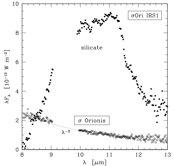
Fig. 2. N -band spectra of \sigma Orionis (circles) and \sigma Ori IRS1 (dots). The spectrum of \sigma Orionis shows a pure photospheric continuum, but the spectrum of \sigma Ori IRS1 exhibits a strong, broad emission feature indicative of silicate dust.
