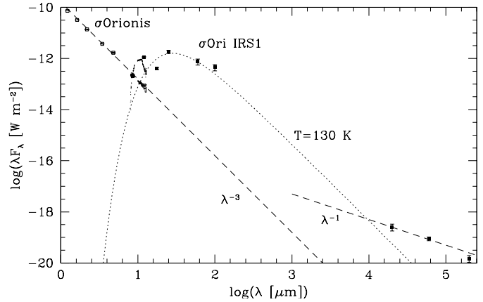
Fig. 3. Spectral energy distributions of \sigma Orionis, purely photospheric, and \sigma Ori IRS1, reproduced by a combination of thermal dust radiation ( T_{\text{dust}} = 130 K) and free-free emission.
