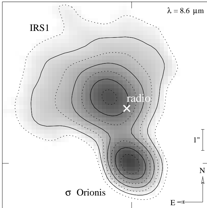
Fig. 1. Mid-infrared image of \sigma Orionis (near the bottom) and IRS1 (near the centre), taken through the N1 -band ( \lambda_0 = 8.6 \mu\text{m} ) filter with the TIMMI-2 camera at the ESO 3.6 m telescope. The position of the radio source as detected by Drake (1990) is indicated by a white cross. The field measures 10'' \times 10'' , with North up and East to the left, and is displayed on a logarithmic scale with a dynamic range of a factor 100.
