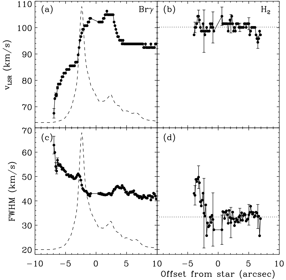
Fig. 4. Spatial variation of the velocity centroid (top panel) and line FWHM (bottom panel) of Br \gamma and H _2 along the symmetry axis of G29.96 (from left to right in Fig. 1). Typical error bars are indicated at different positions along the slit. In panels a ) and c ), the intensity distribution of Br \gamma is plotted (dashed line) for comparison. The dotted lines in panels b ) and d ) represent the average H _2 centroid velocity and FWHM calculated between positions -3'' and +5'' , and 0'' and +5'' , respectively. The zero point along the slit corresponds to the position of the ionizing star. At a distance of 6 kpc, 1'' corresponds to 0.029 pc.
