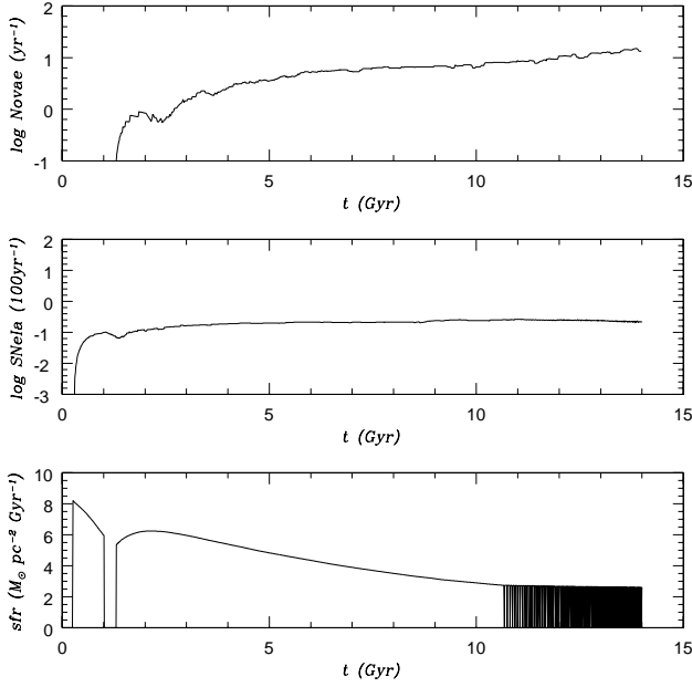
Fig. 1. Nova rate, SNeIa rate and SFR predictions for the “two-infall” model for the Galaxy. Note the oscillatory behaviour of the SFR during the last 2 or 3 Gyr.
