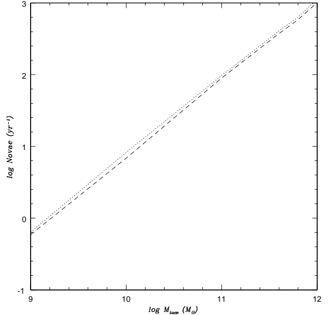
Fig. 4. Ellipticals: nova rate as a function of M_{\text{lum}} of the galaxy: model I (dotted), model II (short-dashed).
