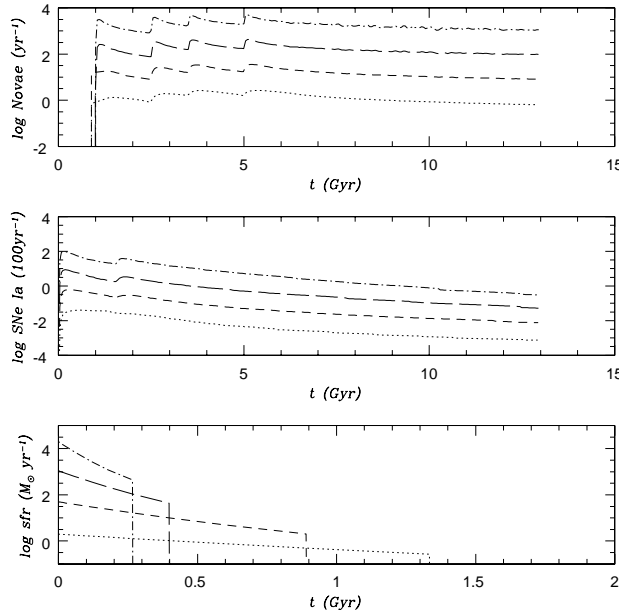
Fig. 2. Ellipticals: star formation rate, SNeIa rate and nova rate predictions for model I. Dotted, 10^9 M_\odot ; short-dashed, 10^{10} M_\odot ; long-dashed, 10^{11} M_\odot ; dotted-short-dashed, 10^{12} M_\odot .
