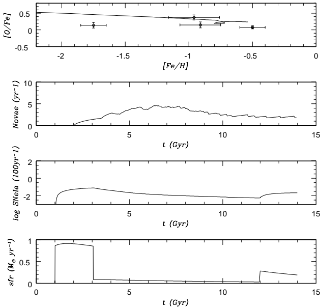
Fig. 5. Irregulars: star formation rate, SNeIa rate, nova rate and [O/Fe] vs. [Fe/H] predictions for the LMC. The data are from Hill et al. (2000).
