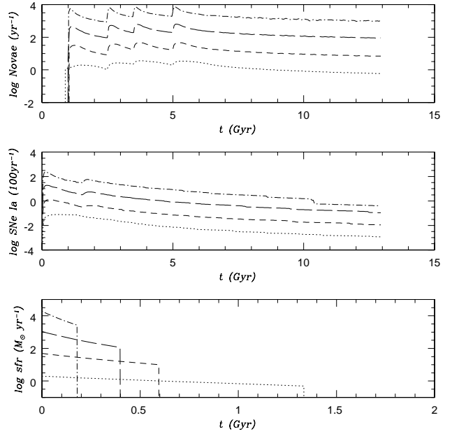
Fig. 3. Ellipticals: star formation rate, SNeIa rate and nova rate predictions for model II. Dotted, 10^9 M_\odot ; short-dashed, 10^{10} M_\odot ; long-dashed, 10^{11} M_\odot ; dotted-short-dashed, 10^{12} M_\odot .
