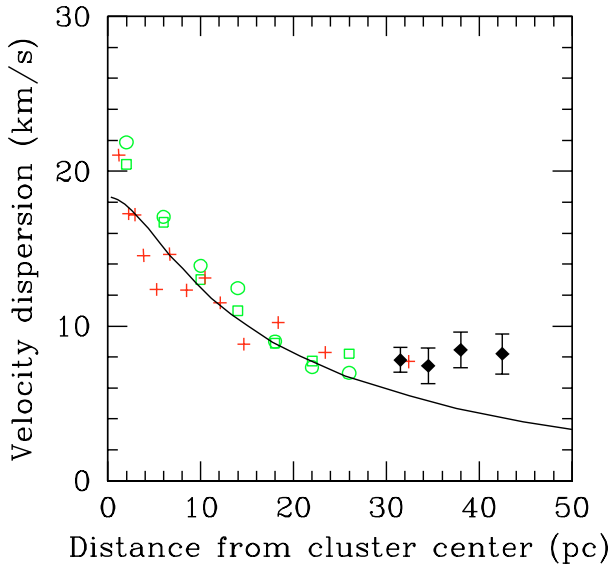
Fig. 1. The velocity dispersion profile of \omega Cen. Proper motion data (Circles and squares) are from van Leeuwen et al. (2000). Radial velocities Crosses are from Meylan et al. (1995) up to 20 pc, while the last two points are from Meylan & Mayor (1986). The solid line is the best fit model of radial velocity data as derived by Meylan et al. (1995) (their Fig. 1). Note the good agreement between the last point of Meylan & Mayor (1986) and our radial velocities measurement (diamonds), which extend the profile to \sim 45 pc.
