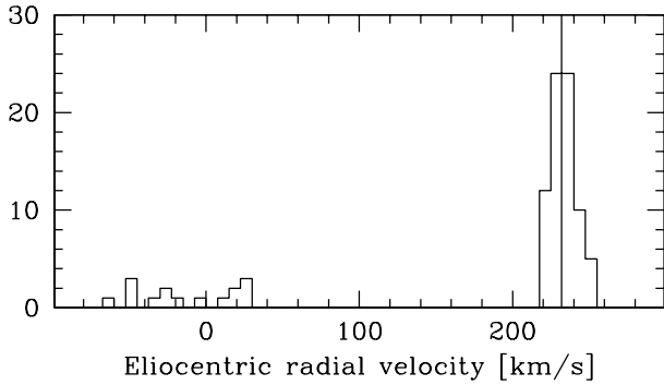
Fig. 2. Distribution of the heliocentric radial velocity for the 91 selected stars. Of all targets, 75 are clearly members having radial velocity comparable to the one of the cluster, marked by a vertical line. The remaining ones are most probably part of the Galactic disk.
