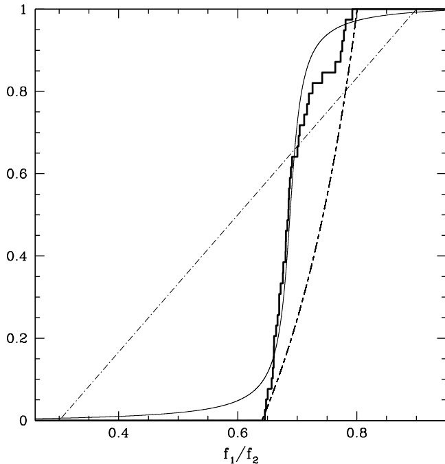
Fig. 1. The cumulative distribution of the frequency ratio of the twin kHz QPOs in Sco X-1 and three theoretical models. Dot-dashed line: a uniform distribution in the range (0.3, 0.9); dashed line: beat frequency model with upper frequency distributed uniformly in the range (872 Hz, 1081 Hz); thin continuous line: the best fit Lorentzian. Of the three models, only the Lorentzian fits the data.
