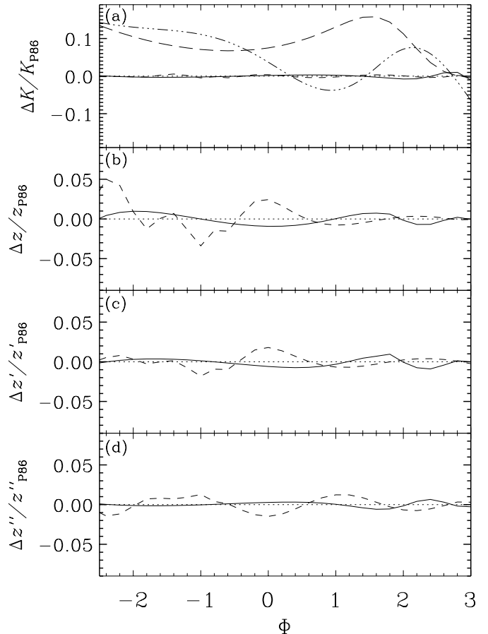
Fig. 2. The relative difference of K a ), z b ), z' c ) and z'' d ) between our analytic fits and the values calculated by P86. The solid line represents the case of a repulsive potential, the short-dashed one the case of an attractive potential; the dotted line indicates the line of zero difference. Also shown in a ) is the difference between the IM85's and P86's results (long-dashed) and IM85's and M84's results (dash-dot-dotted line).
