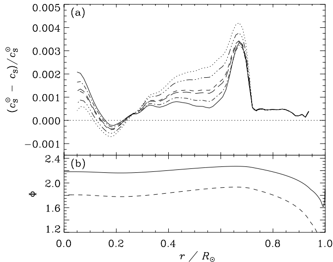
Fig. 3. a) The relative difference between the seismic model of Basu et al. (1997) and solar models computed with different resistance coefficients: S1 (solid line), S2 (dotted), S3 (dash-dot-dot-dotted), S4 (short-dashed), S5 (long-dashed) and S6 (dash-dotted). The resistance coefficients used in the models are summarized in Table 2. b) The run of \Phi for H^+ - H^+ (solid) and He^{2+} - He^{2+} collisions (dashed line) in solar models.
