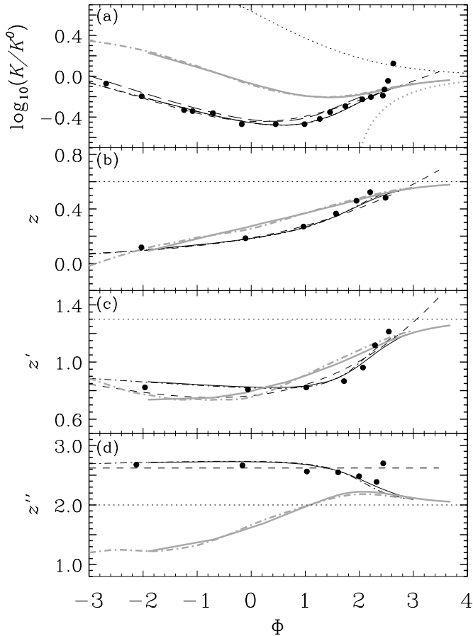
Fig. 1. The resistance coefficient K a ), z b ), z' c ) and z'' d ) as computed by B69 (dotted), MMS67 (solid), M84 (short-dashed), P86 (dash-dotted) and IM85 (long-dashed line). The dark black lines indicate the case of repulsive potentials, while the brighter ones show the values for attractive forces (not computed by M84 and IM85). The dots represent the actual values computed by M84.
