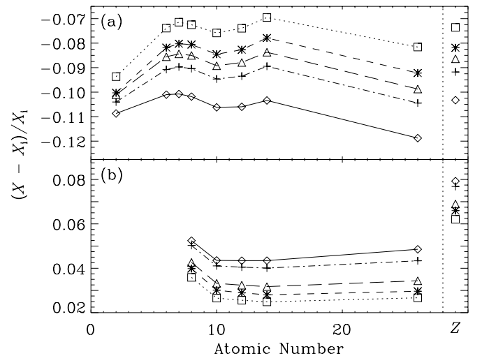
Fig. 4. a) The surface depletion of various elements in solar models with different collision integrals from the pre-main sequence until now. The line-styles correspond to Fig. 3. On the right hand side the change in the overall metallicity is shown. b) Like a), but for the centre.
