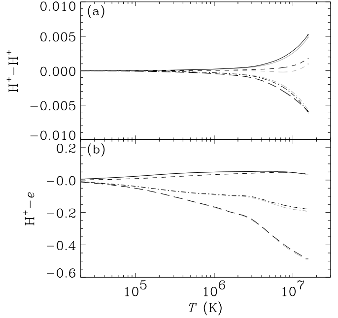
Fig. 5. a) The relative change of K (long-dashed line), z (solid), z' (short-dashed) and z'' (dash-dotted) for \text{H}^+ - \text{H}^+ collisions in the Sun in the sense (quantum – classical)/classical. For the dark line the quantum corrections tabulated by H71 have been utilized, while the grey lines were obtained with our fitting formulae (see Appendix A). b) As a) , but for \text{H}^+ - e collisions.
