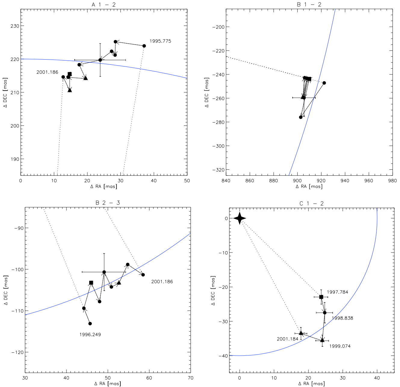
Fig. 2. Relative motion in the systems \theta^1 Ori A1–2, \theta^1 Ori B1–2, \theta^1 Ori B2–3, and \theta^1 Ori C1–2. The brighter component is always placed at the origin (0, 0) of the plot. The solid symbols represent the observed positions of the companion over time from Table 2; J -band data are shown by triangles, H -band data by squares, and K -band data by circles. For clarity we show error bars in each plot for one data point only. In the plot for \theta^1 Ori C1–2 we show error bars for all four orbital points, and we also mark the primary position by a big asterisk. In each plot the first and last positional measurements in the data series are connected to the origin by a thin dotted line. The solid line shows a part of a circle around the primary position.
