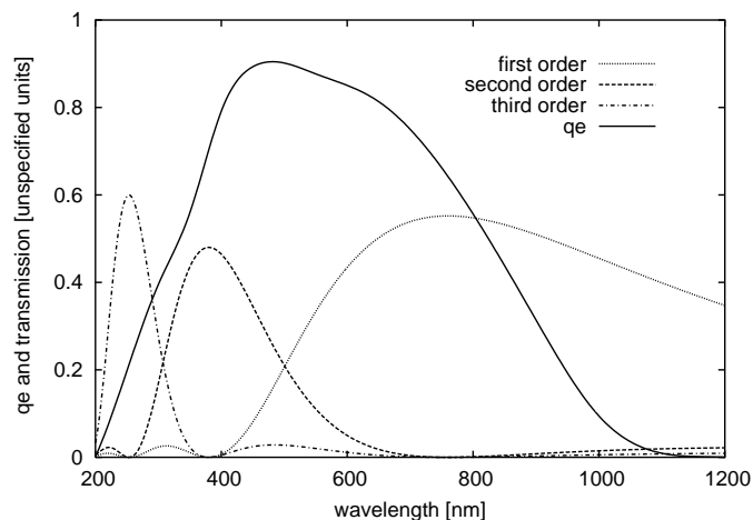
Fig. 2. Transmission curves for the first, second and third grating orders, plus the quantum efficiency. The order’s curves have been scaled down by a factor of 0.6 to better represent data from the real grating.
