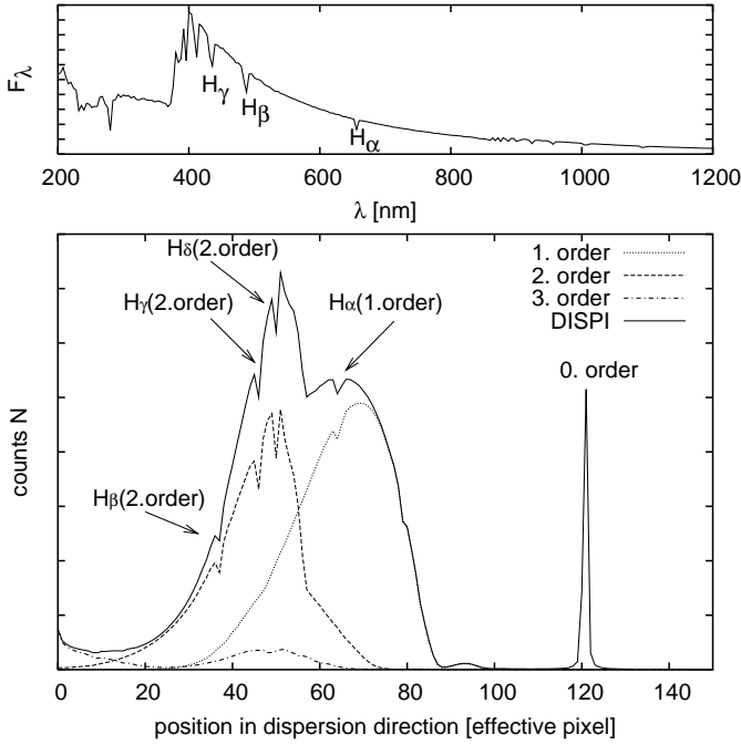
Fig. 4. Input spectrum (top) and simulated DIVA DISPIS (bottom) for a star with T_{\text{eff}} = 9500 K, \log g = 4 , solar metallicity (without noise, as in Fig. 3). Here the H_{\alpha} , H_{\beta} and H_{\gamma} features are marked in the model spectrum as well as in the resulting DISPIS. For such a star, the third order starts to contribute to the signal.
