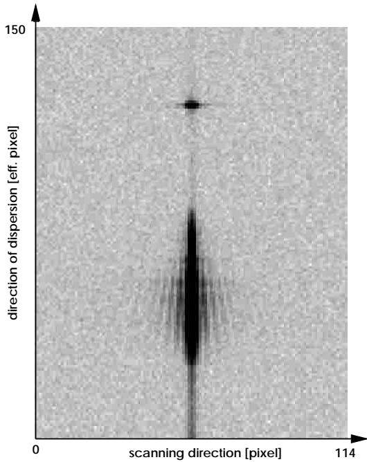
Fig. 5. A dispersed image for an M type star, V = 10 mag (with noise) as generated by the simulation software from Scholz (1998). Note the contribution of the zeroth order seen as a single intensity “blob” in the upper part of the image. The first, second and third spectral order are all overlapping (lower intensity “stretch”) due to the grating. The intensity stripes to the side of the dispersed image are due to diffraction at the telescope’s aperture.
