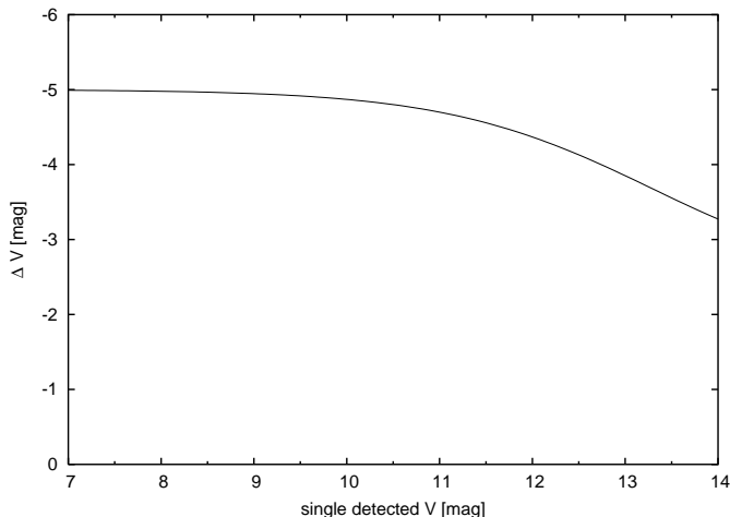
Fig. 6. One-hundred added frames each of the “single” visual magnitude given on the x -axis yield the same S/N as a star which is \Delta V magnitudes brighter. For example, adding 100 frames of V = 14 mag stars (two-dimensional intensity distributions) and calculating a DISPIS from these yields a DISPIS which has the same S/N as a single DISPIS of a star with V = 10.8 mag. Clearly, for fainter stars, the noise is dominated by the read-out noise, while for brighter stars only the Poisson noise of the signal is relevant, thus yielding a full magnitude shift of 5 mag. This curve was calculated by making use of the specific DIVA’s CCDs noise characteristics.
