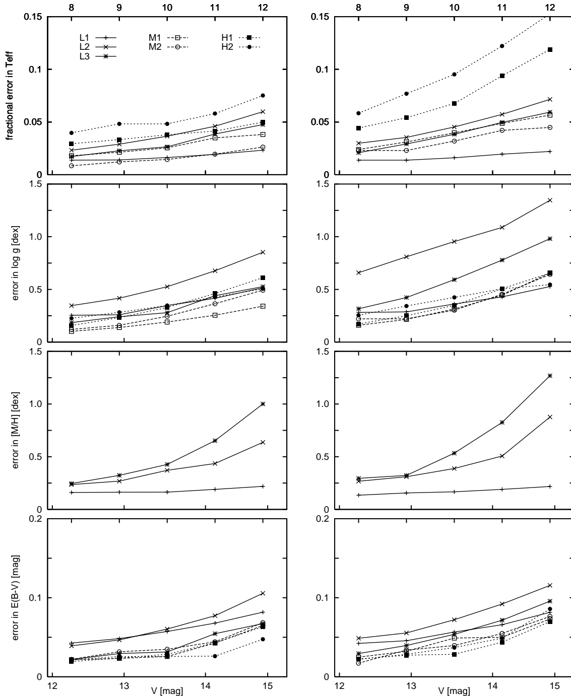
Fig. 8. The same as in Fig. 7 but with extinction included. The left column shows the results for networks which were trained with UV data while the right column shows the classification results for tests without UV data.
