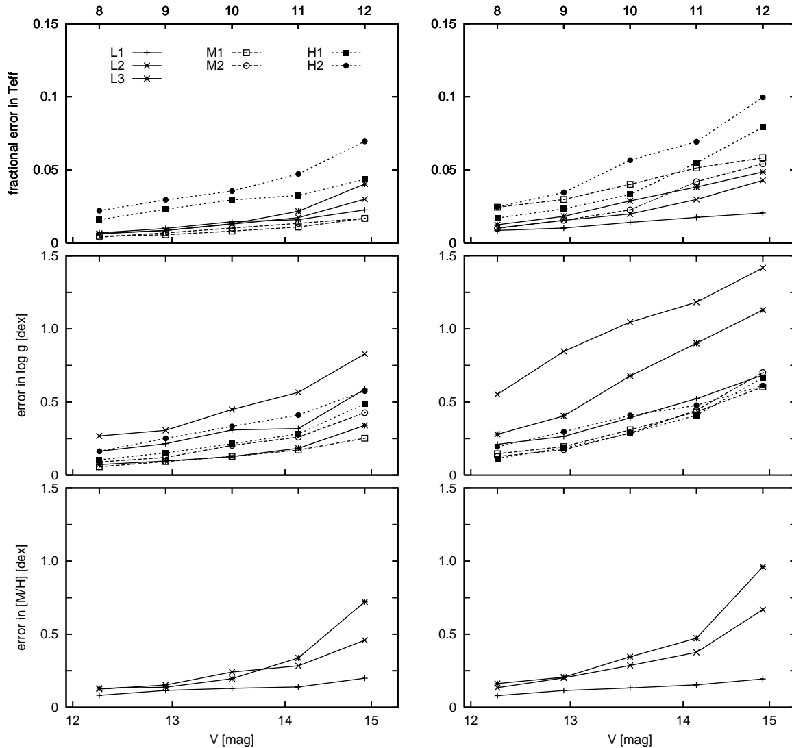
Fig. 7. The average classification uncertainty for T_{\text{eff}} , \log g and [M/H] from top to bottom as a function of visual magnitude, V , plotted for the different temperature sets. No extinction was added for these simulations. The stated error is that of Eq. (1). The lower magnitude scale refers to end of mission data in which 100 DISPIS of objects with the magnitude given on the upper scale are stacked (see Fig. 6 for details). The lettering for the different temperature ranges refers to the temperature ranges given in Table 2. The left column shows the results for networks which were trained on DISPIS (with an effective pixel range from 30 to 80) including the UV channel fluxes for the particular star, while the right column shows results for those simulations without UV data. For [M/H] only the results for the temperature ranges L_1 to L_3 and [M/H] \geq -0.3 dex are presented, as for higher temperatures and lower metallicities spectral information of this parameter is washed out at these resolutions.
