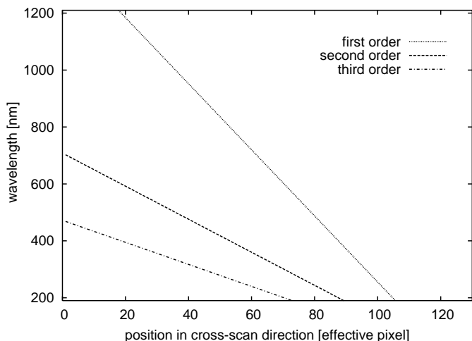
Fig. 1. Wavelength versus position on the spectroscopic CCD (SC) for the first, second and third order. The zeroth order which is made up of undispersed (white) light would lie at about pixel position 122, but is not shown.
