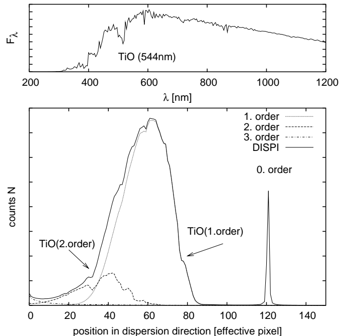
Fig. 3. Input spectrum (top) and simulated DIVA DISPIS (bottom) for a star with T_{\text{eff}} = 4500 \text{ K} , \log g = 4 and solar metallicity (no noise added). Top: the model spectrum sampled in steps of 4 nm, which matches roughly the resolution of the third order of the DIVA dispersed image, shows spectral structure of which the TiO band is marked. Bottom: DIVA DISPIS showing total counts (in arbitrary units) detected along the effective pixels in the extracted DIVA dispersed information. The TiO feature of the input spectrum (top) can be recognized in the contributions to the first and second orders.
