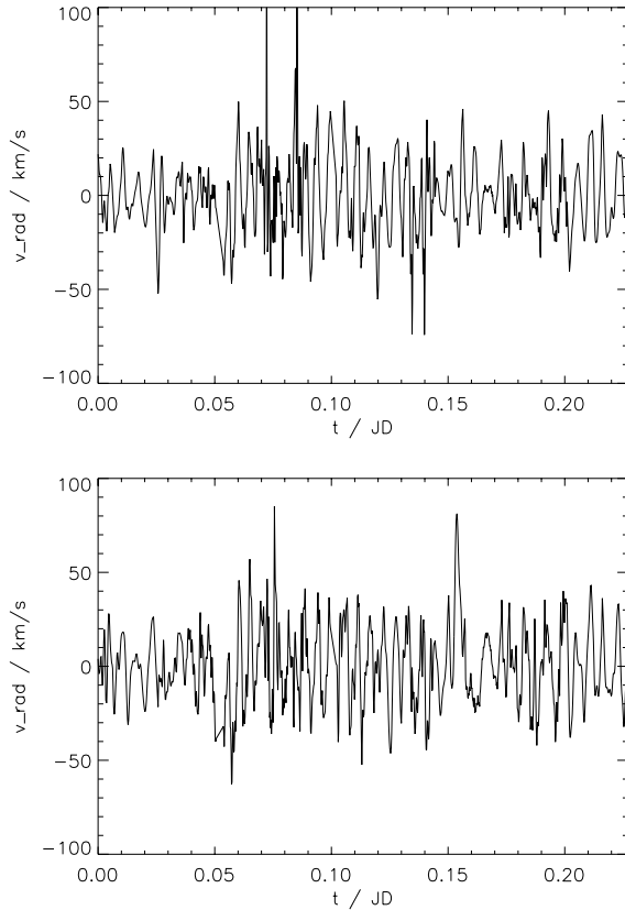
Fig. 2. Radial velocity curve for H_\beta (upper panel) and H_\gamma (lower panel); artefacts due to poor weather conditions were not removed.
