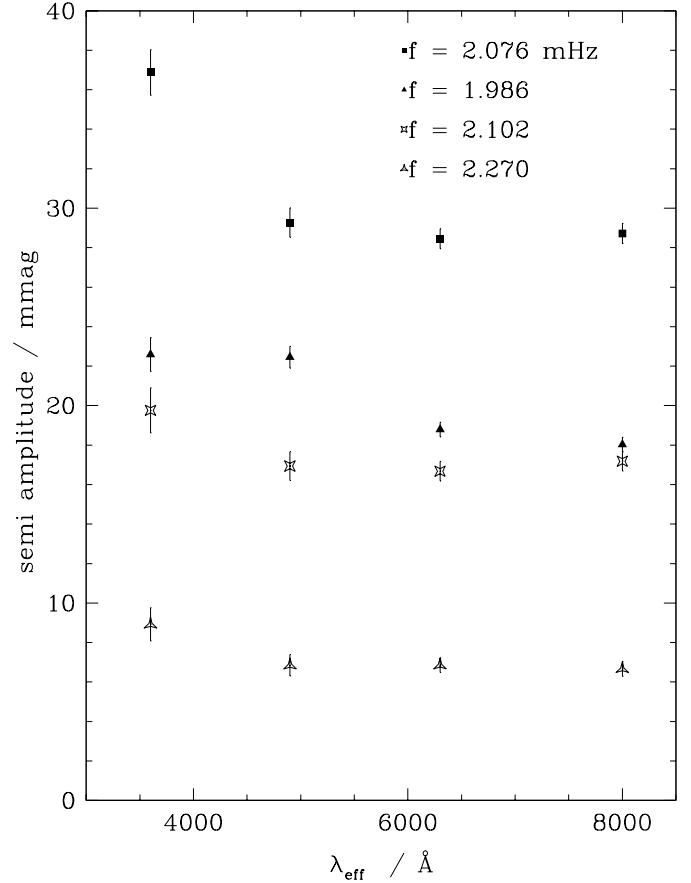
Fig. 5. Semi amplitudes of four frequencies as a function of effective wavelength. The error bars are 1\sigma errors and are calculated by means of a \chi^2 method.
