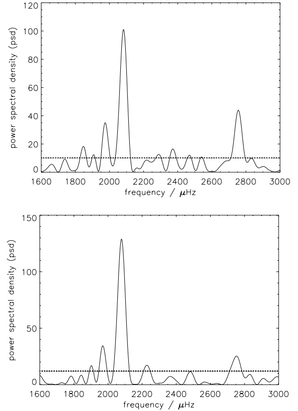
Fig. 3. Lomb-Scargle periodogram of the radial velocity curve of H_\beta (upper panel) and H_\gamma (lower panel). The power spectral density (psd) is a measure for the probability that a period is present in the radial velocity curve or light curve. The horizontal line represents the confidence level of 99% ( 3\sigma -level).
