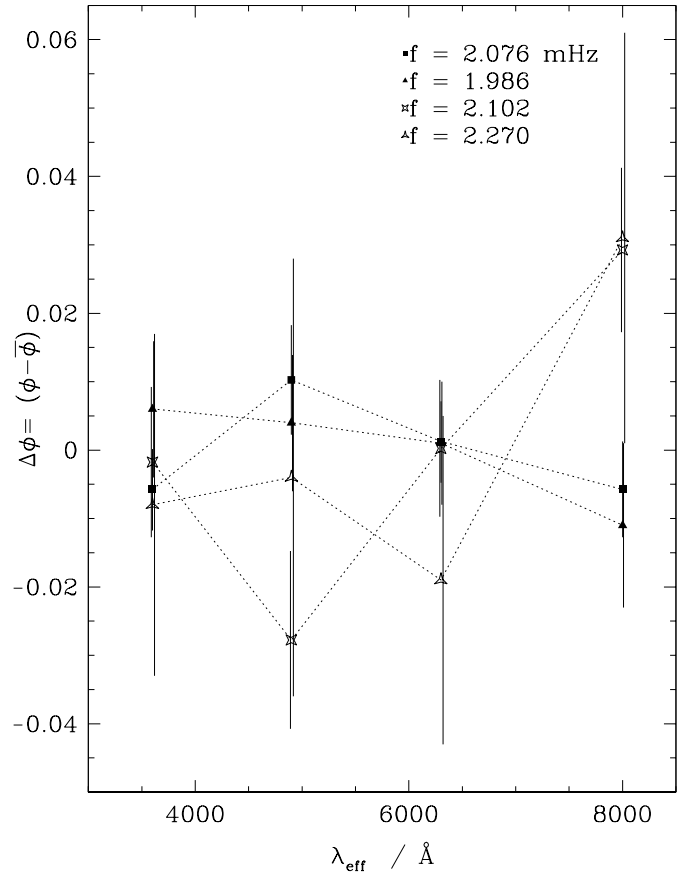
Fig. 7. Deviation of the phases from the mean value calculated from the four frequency bands for the frequencies given in Fig. 5. The error bars are calculated from the amplitude errors as described in the text.
