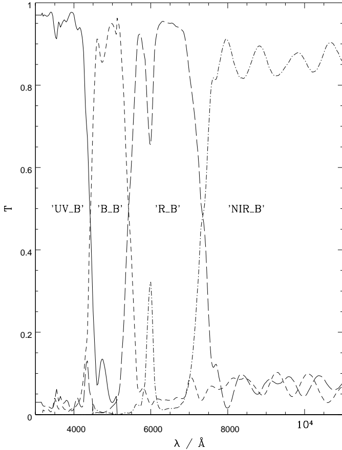
Fig. 1. Transmission curves of the four BUSCA wavelength bands. The four ranges are denoted by “UV B ” (central wavelength: 3600 Å), “B B ” (4800 Å), “R B ” (6300 Å) and “NIR B ” (8000 Å) although these are not comparable to the classical Johnson UBVRI system.
