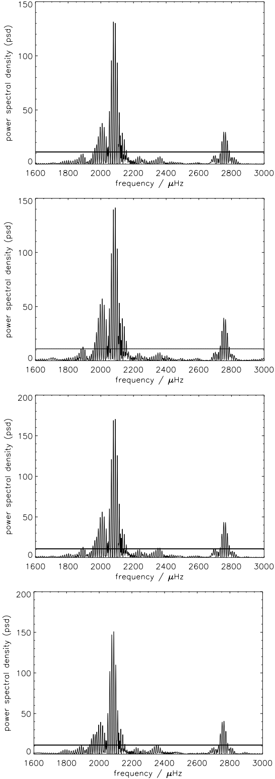
Fig. 4. Lomb-Scargle periodogram of the light curves of the “ UV_B ”, “ B_B ”, “ R_B ” and “ NIR_B ” band (from top to bottom) of the BUSCA camera. The horizontal line in each panel represents the confidence level of 99% ( 3\sigma -level).
