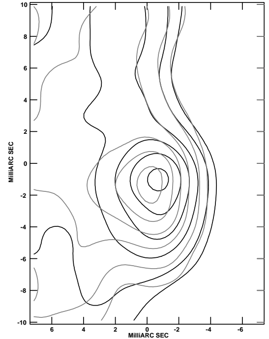
Fig. 4. Overlay of the hot spot region in the west lobe (W1). Contours are drawn in grey (epoch 1995.554) and black (epoch 2000.504) at 1, 2, 4, 6, 8, 10 mJy/beam. The two images have been aligned on the position of the east hot spot E2.
