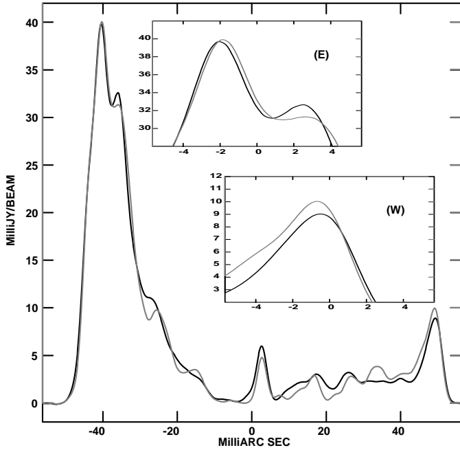
Fig. 5. A slice through the hot spots of 4C 31.04. The central small peak results from the northern edge of the core (the hot spots are not perfectly symmetric about the core). The black line shows the profile of the 2000.504 image, while the grey line represents the profile of the 1995.554 image. Shown inset are magnified versions of the profile at the east (E) and west (W) hot spots.
