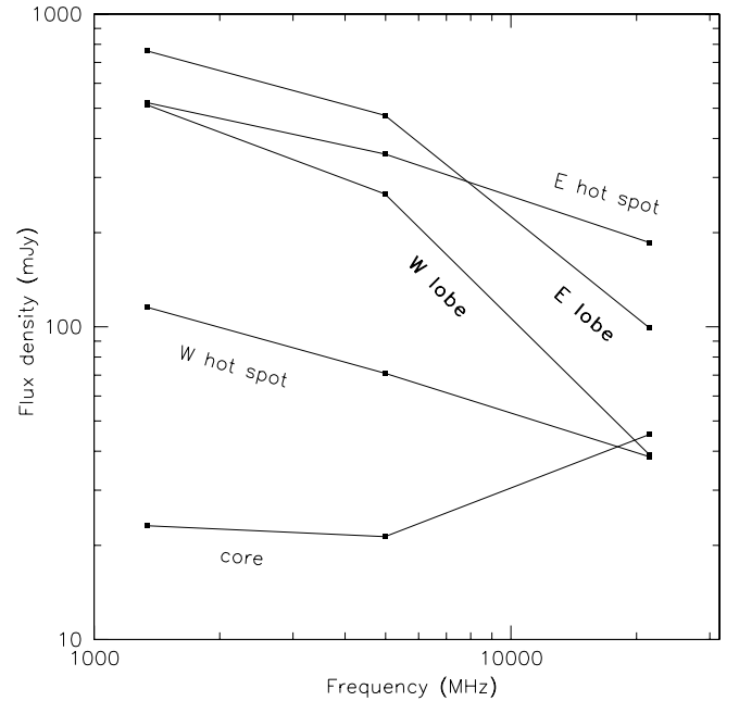
Fig. 8. The spectrum of lobes, hot spots and core. The steepening of both lobes is clearly visible above 5 GHz.
