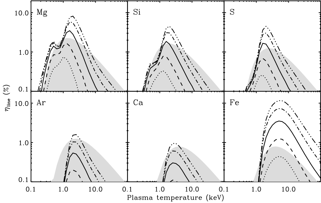
Fig. 1. Efficiency of K_\alpha line emission for several elements as a function of the temperature in an optically thin plasma. The parameter \eta_{\text{line}} is defined as the line luminosity over the bolometric luminosity of the thermal plasma. Each panel shows 5 different lines. From top to bottom these refer to a metallicity 10, 3, 1, 0.3 and 0.1 solar. The gray shading highlights regions in the parameter space where an equivalent width lower than 100 eV is predicted.
