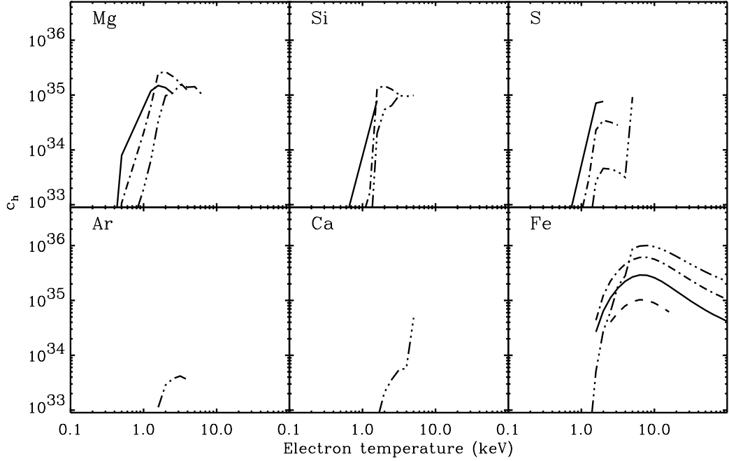
Fig. 4. The luminosity coefficient c_h (see text) as a function of the plasma temperature and of metallicity for the considered elements. As in Fig. 1, the dotted, dashed, solid, dot-dash and dot-dot-dot-dash lines are relative to 0.1, 0.3, 1, 3 and 10 time solar metallicity, respectively.
