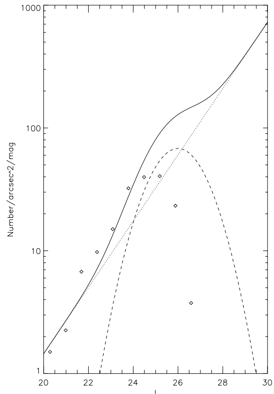
Fig. 1. We show NGC 564 external source luminosity function between 14'' and 23'' from the center of the galaxy. The solid line shows the sum of the globular cluster luminosity function plus the background galaxy luminosity function. The dashed line shows the fitted globular cluster luminosity function, the dotted line the background galaxy luminosity function.
