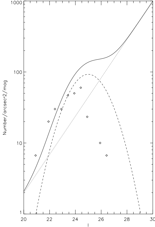
Fig. 2. We show NGC 7619 external source luminosity function between 20'' and 52'' from the center of the galaxy. The solid line shows the sum of the globular cluster luminosity function plus the background galaxy luminosity function. The dashed line shows the fitted globular cluster luminosity function, the dotted line the background galaxy luminosity function.
