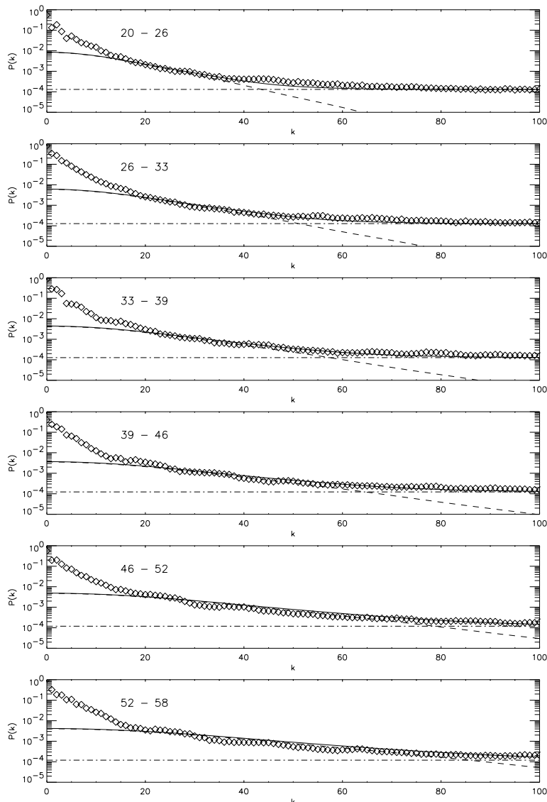
Fig. 4. NGC 7619 SBF measurement. We show NGC 7619 power spectrum as was fitted in six different annuli of width \approx 6'' . The fit of the power spectrum is given by the solid line, the PSF power spectrum by the dashed line and the dashed-dotted line is the fitted constant white noise spectrum.
