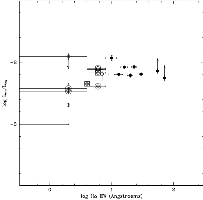
Fig. 4. L_{C\ II}/L_{FIR} vs. the equivalent width of the H\alpha line, H\alpha EW . L_{C\ II} is corrected for the LWS aperture. Only the 19 galaxies with available measurements are plotted. The galaxy out of bounds is NGC 4491, with H\alpha EW consistent with 0 Å. The non-linear relation between L_{C\ II}/L_{FIR} and H\alpha EW found by P99 is confirmed.
