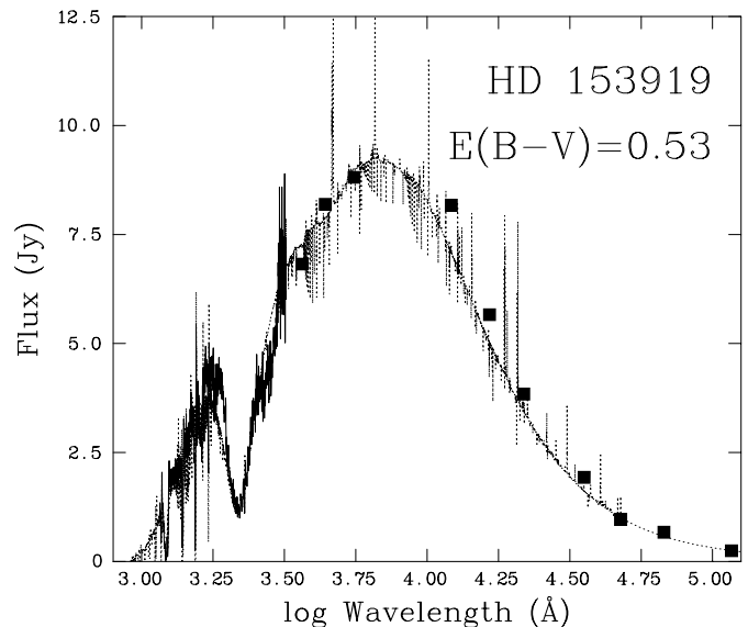
Fig. 2. Plot of the observed (solid line and data points) and theoretical (dotted line) UV-mid-IR spectral energy distribution for HD 153919.
