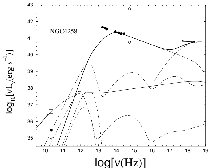
Fig. 2. Model fit to the spectrum of NGC 4258. The parameters are chosen to fit the XMM-Newton result. The lines are defined as in Fig. 1. The discrepancy in the mid-IR may be due to variability (see text for details).
