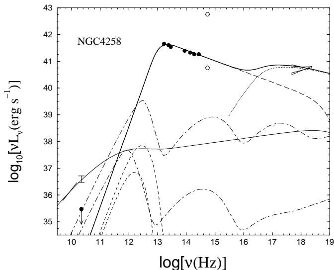
Fig. 1. Model fit to the spectrum of NGC 4258. Parameters are chosen to fit the BeppoSAX data, which is described in Sect. 2. The thick solid line shows the emission from the radiative shock at the base of the jet, with the long-dashed and dotted lines being for the synchrotron and its self-Comptonized emission, respectively (Sects. 3.1 and 3.2). The thin solid line shows the emission from the outer part of the jet (Sect. 3.3). The dot-dashed and short-dashed lines are for the underlying ADAF and SSD, respectively, with two different accretion rates, and are minor contributors to the spectrum.
