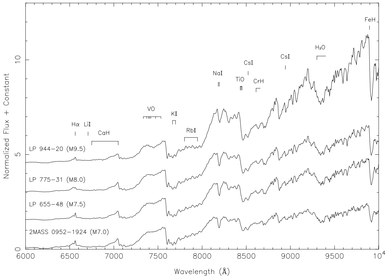
Fig. 1. ESO 3.6-m/EFOSC2 spectra of LP 775-31 and LP 655-48, compared with those of LP 944-20, a known M9.5 brown dwarf (Tinney 1996, 1998; Reid et al. 2002b), and the M7.0 dwarf 2MASS 0952219–192431 (Gizis et al. 2000). An arbitrary constant has been used to separate the spectra. The location of features typical of late-type stars are labelled, including metal oxide and hydride absorption bands, atomic absorption lines, lithium absorption, and H\alpha emission.
