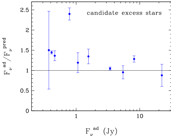
Fig. 4. The properties of the stars more than 3\sigma away from the peak of the distribution presented in Fig. 3. The error bars present \pm 3 \times \Delta F_{\nu}^{\text{ad}} . The star HD 39060 ( \beta Pic) is not included due to its off-scale positive excess of a lot.
